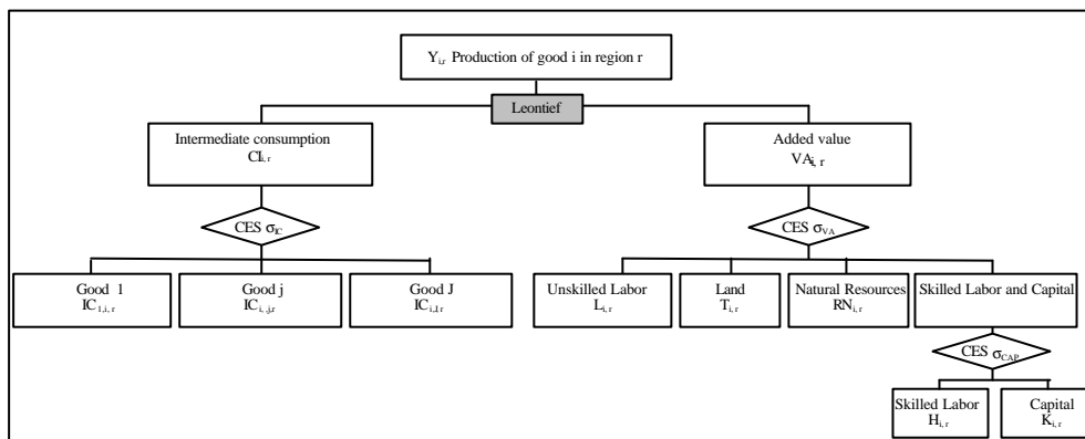
Figure 2: Structure of sector's i production function
