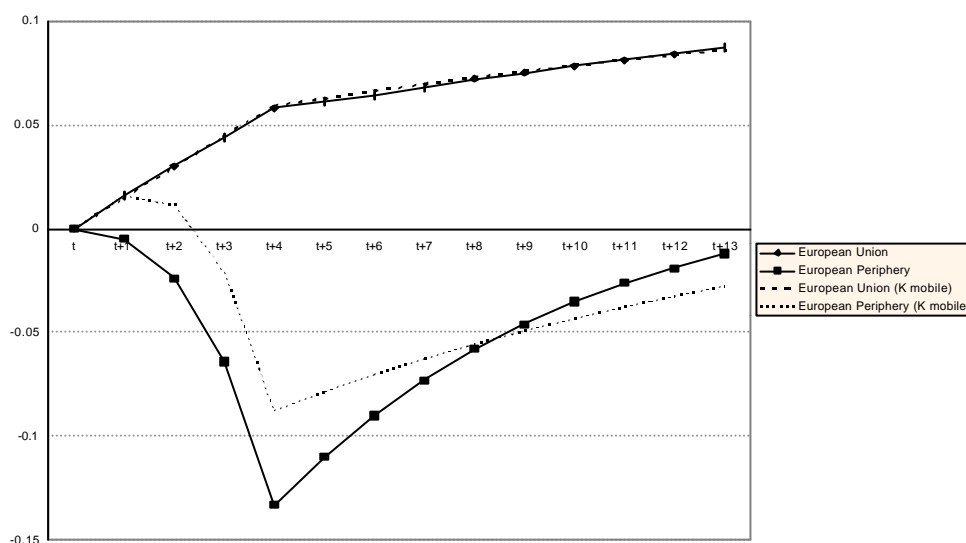
Graph 1: Impact on welfare in the EU and its periphery (%)
