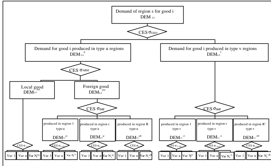
Figure 1: Demand nesting for good i
