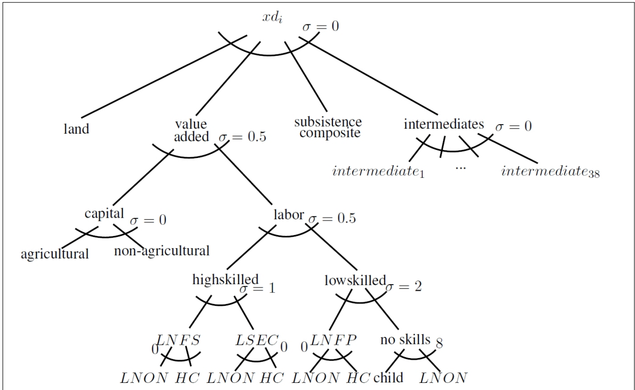
Figure 1: Nested production function
