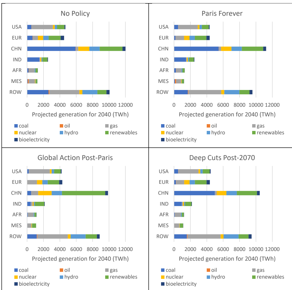
Figure 6. Global generation projection for 2040 by region
