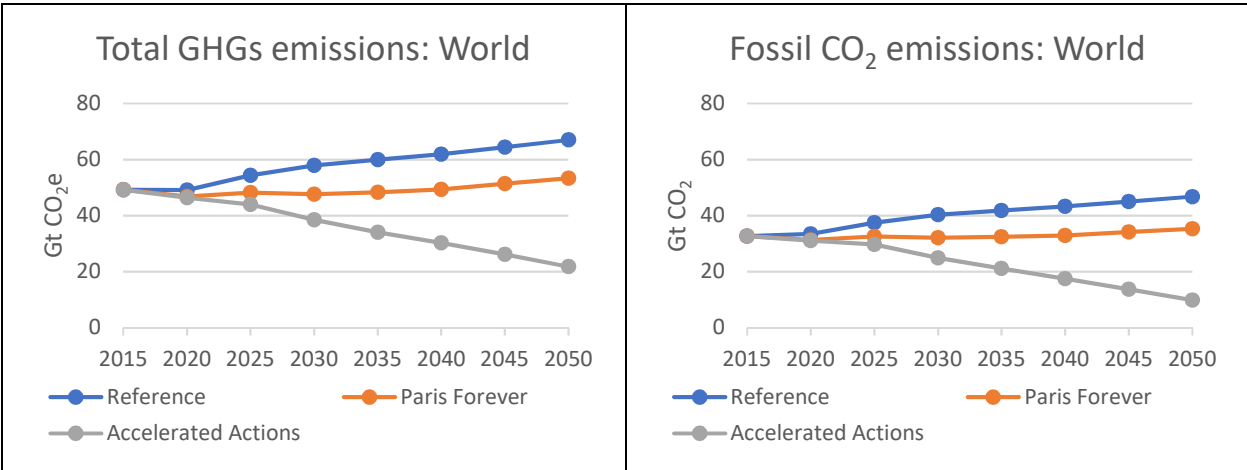
Figure 11. Projections for global GHGs and fossil CO 2 emissions
