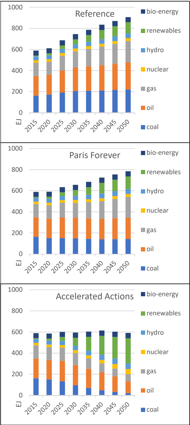
Figure 13. Projections for global primary energy use
