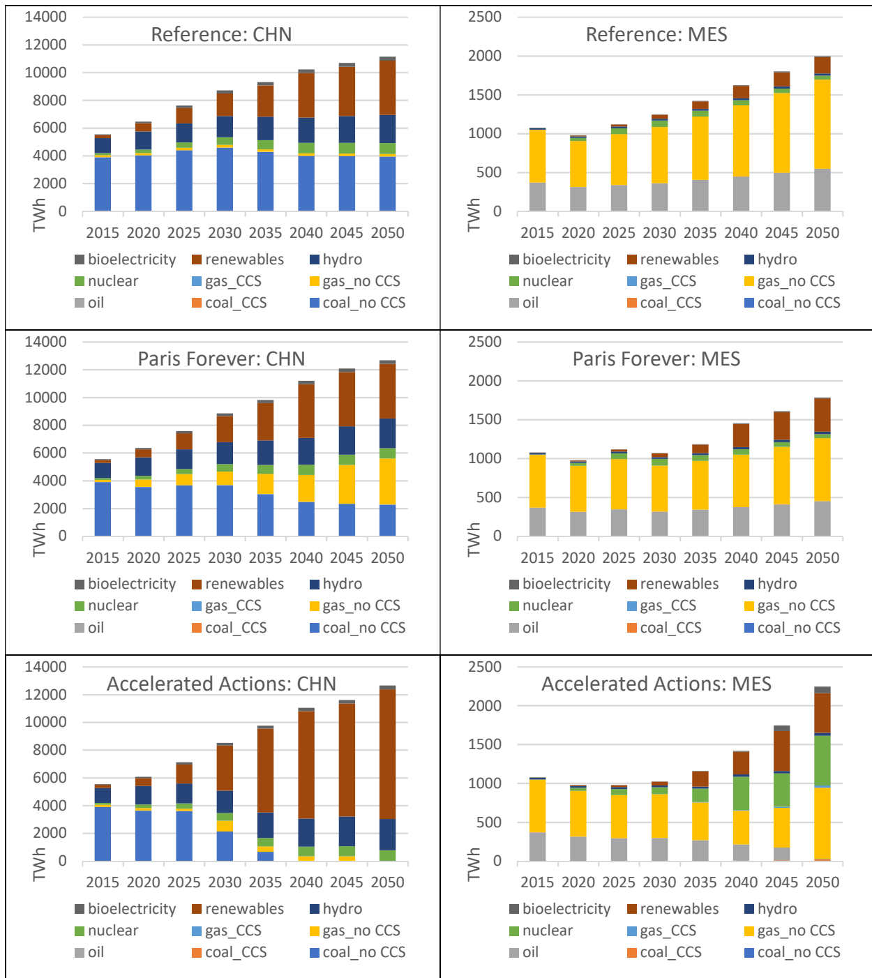
Figure A13-1. Projections for regional generation mix (continued)
