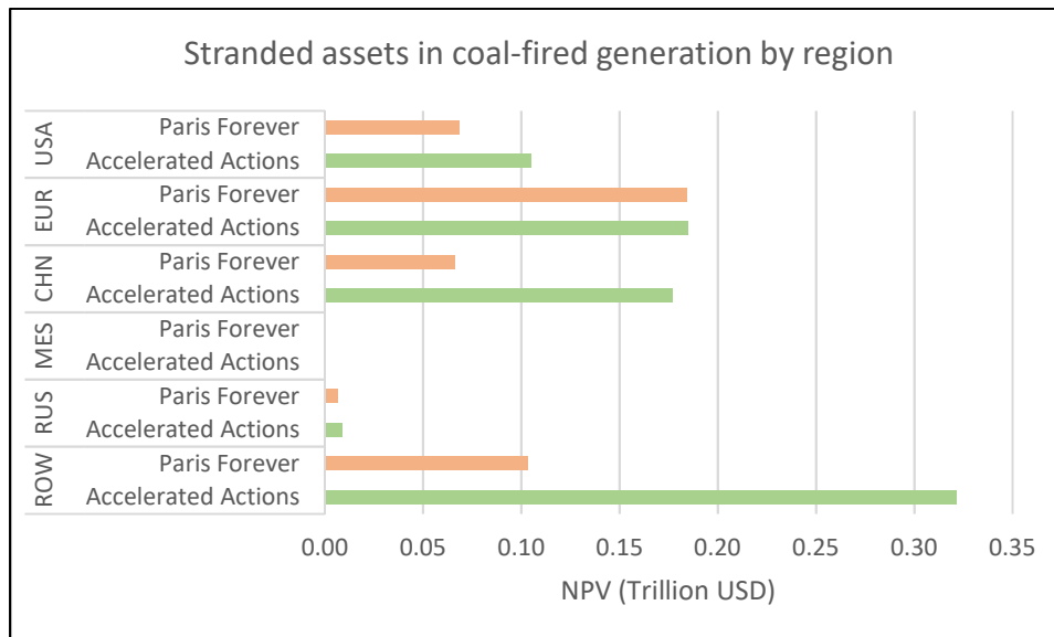
Figure 22. Stranded capital of coal-fired generation relative to the reference scenario by region.
