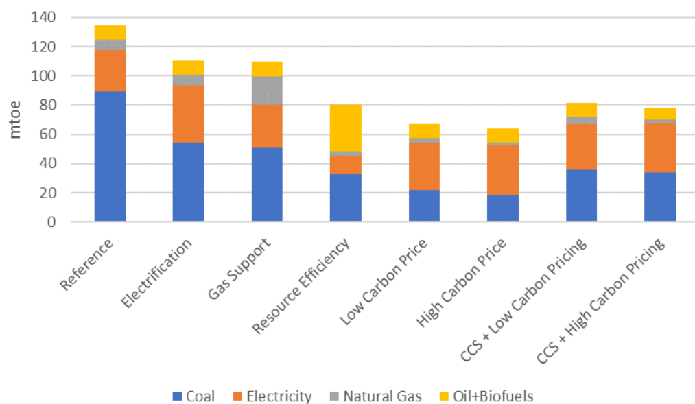
Figure 12. Energy Use in Steel Production in 2050.
