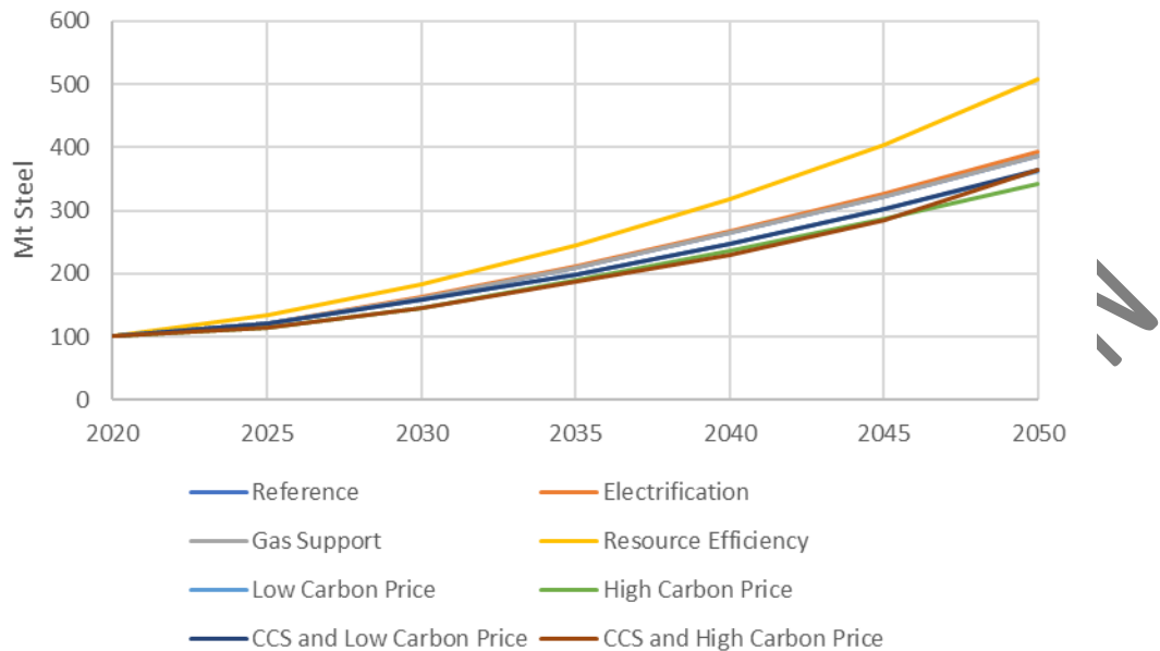
Figure 9. India's Steel Production in Different Scenarios.
