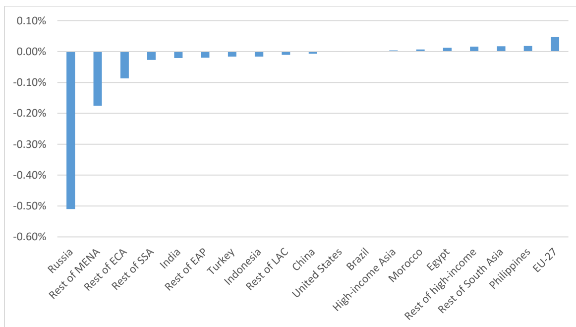
Figure 3.8. Changes in real income under the EU CBAM scenario in 2050, percent difference w.r.t. NDC scenario
