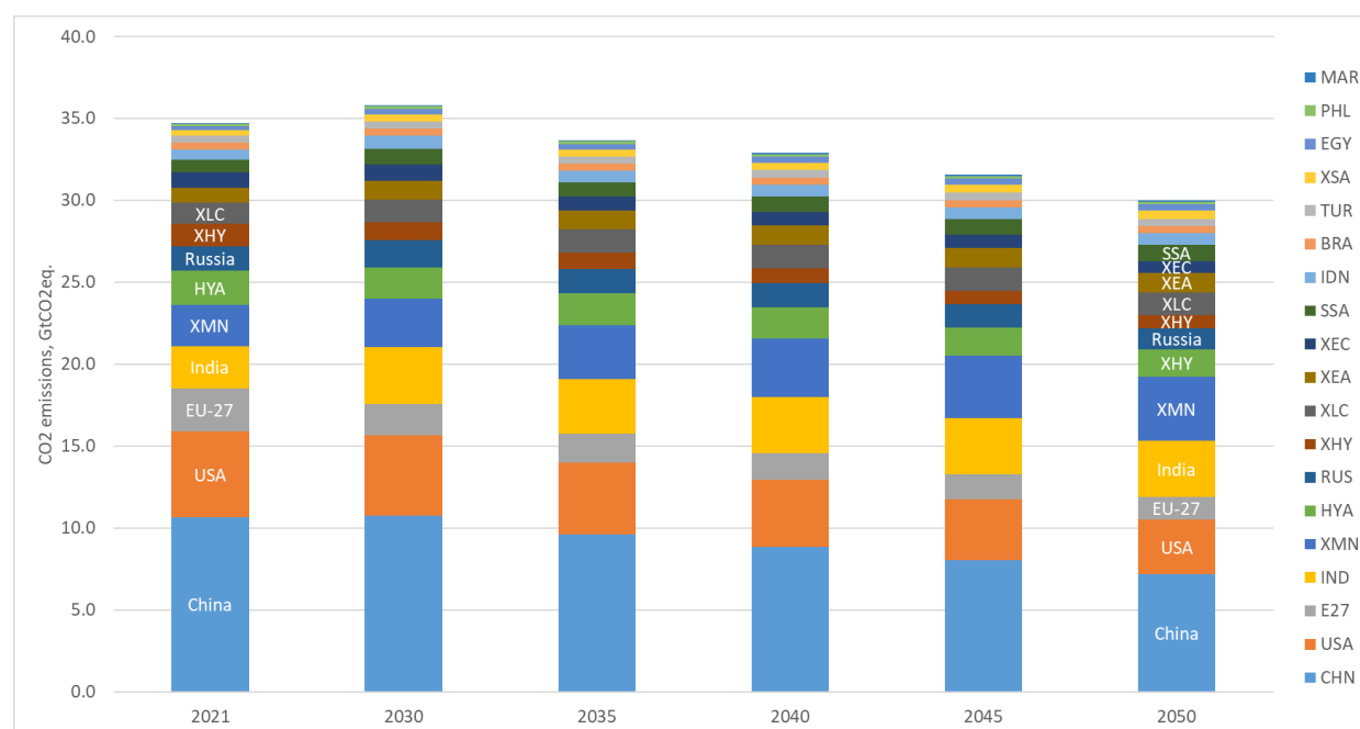
Figure 3.5. CO 2 emissions by regions and years under the NDC scenario, Gigatonnes (Gt) of CO 2 eq.
