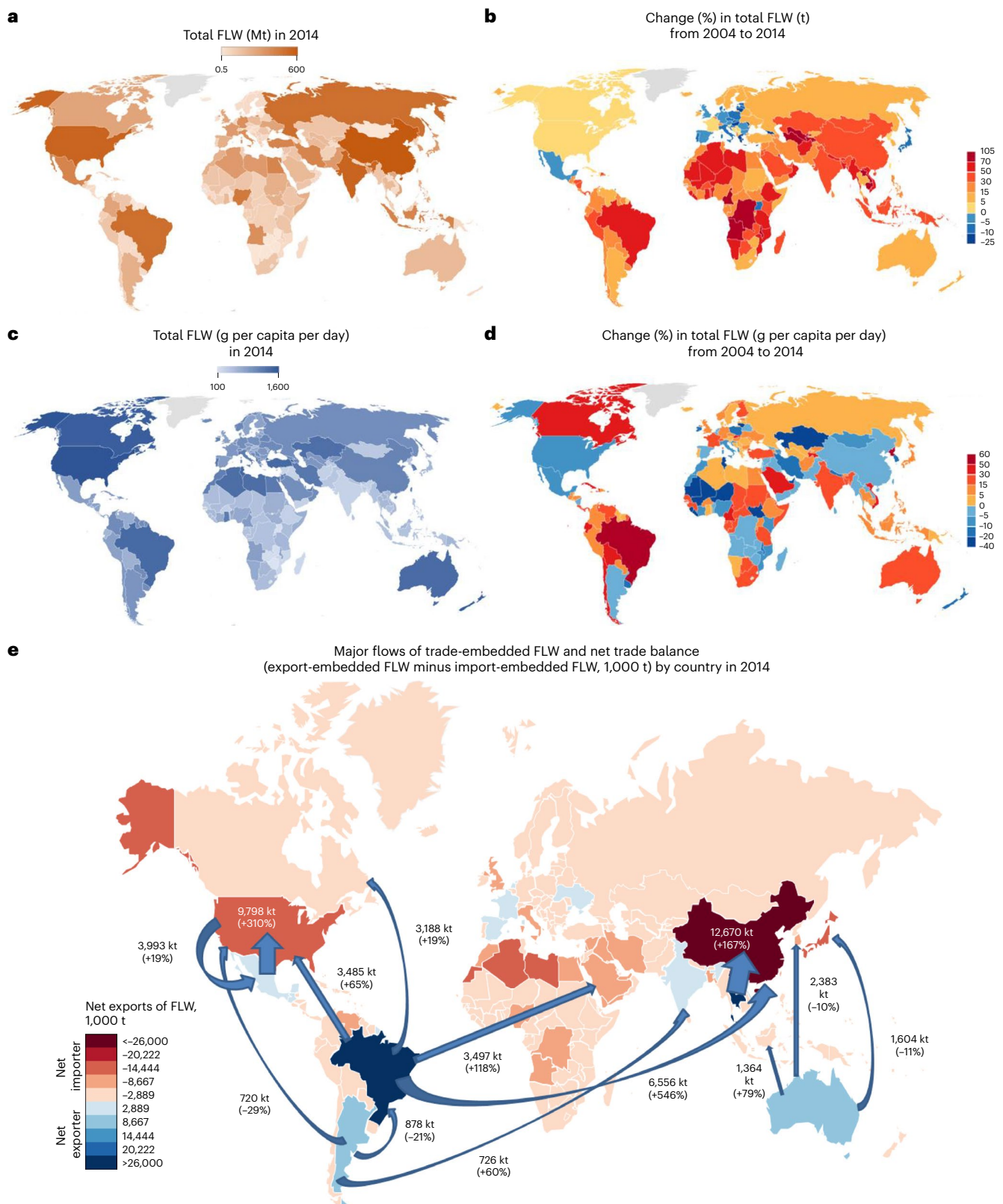
Fig. 2 | Total FLW generation, per capita FLW generation and trade-embedded FLW by country. Estimates reported in the figure refer to FLW generation and are specified in different metrics according to the panel. a , Total FLW generation (million tonnes) by country in 2014. b , Changes (%) in total FLW generation by country in the time period between 2004 and 2014. c , FLW generation (grams per capita per day) by country in 2014. d , Changes (%) in grams per capita per day FLW generation between 2004 and 2014 by country. e , Major global flows of trade-embedded FLW across global regions (1,000 t and change (%) with respect to
