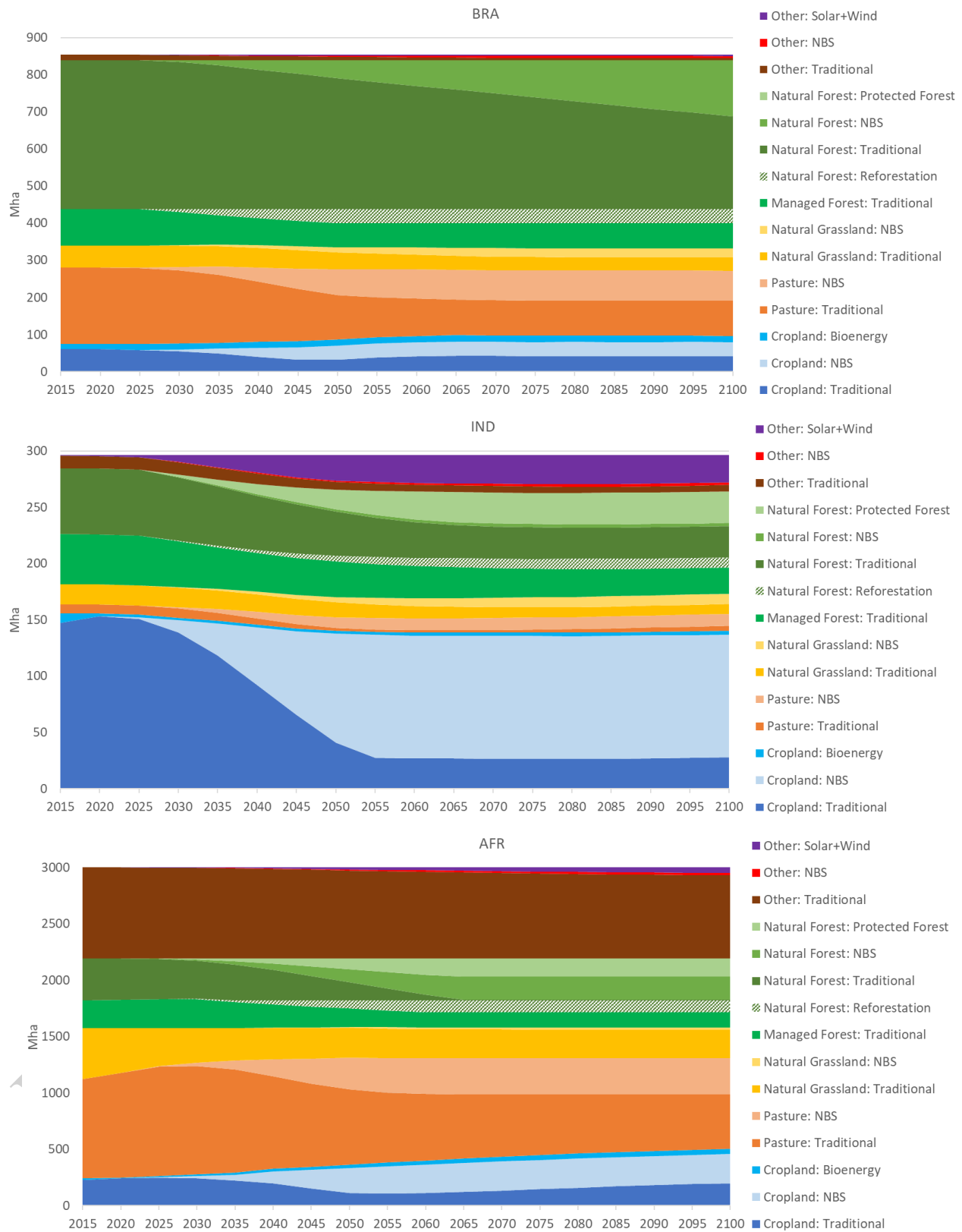
Figure 8. Land use evolution (2015-2100) in selected regions (USA, Europe, China, India, Brazil, Africa). Source: authors calculations.
