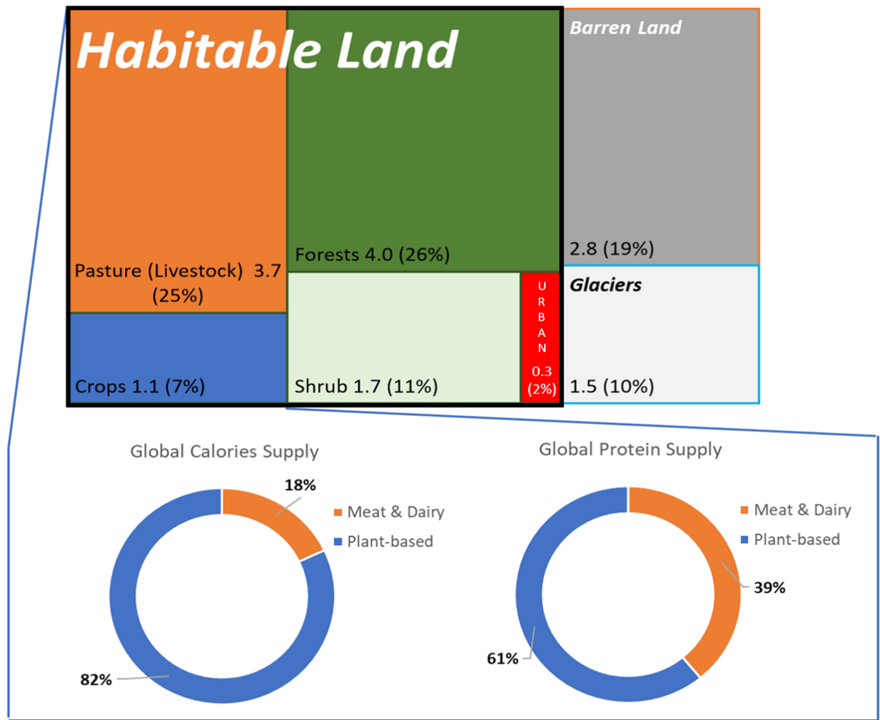
Figure 1. Current global land use (in gigahectares, Gha, and percentage of total) by land category and shares of animal and plant-based sources in global supply of calories and protein. Data source: Ritchie and Roser (2013), FAO (2019).
