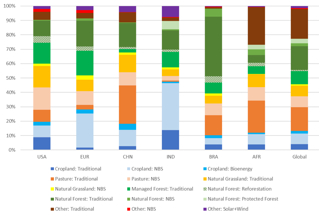
Figure 9. Comparison of 2050 land use shares (%) in selected regions (USA, Europe, China, India, Brazil, Africa, and The World). Source: authors calculations.
