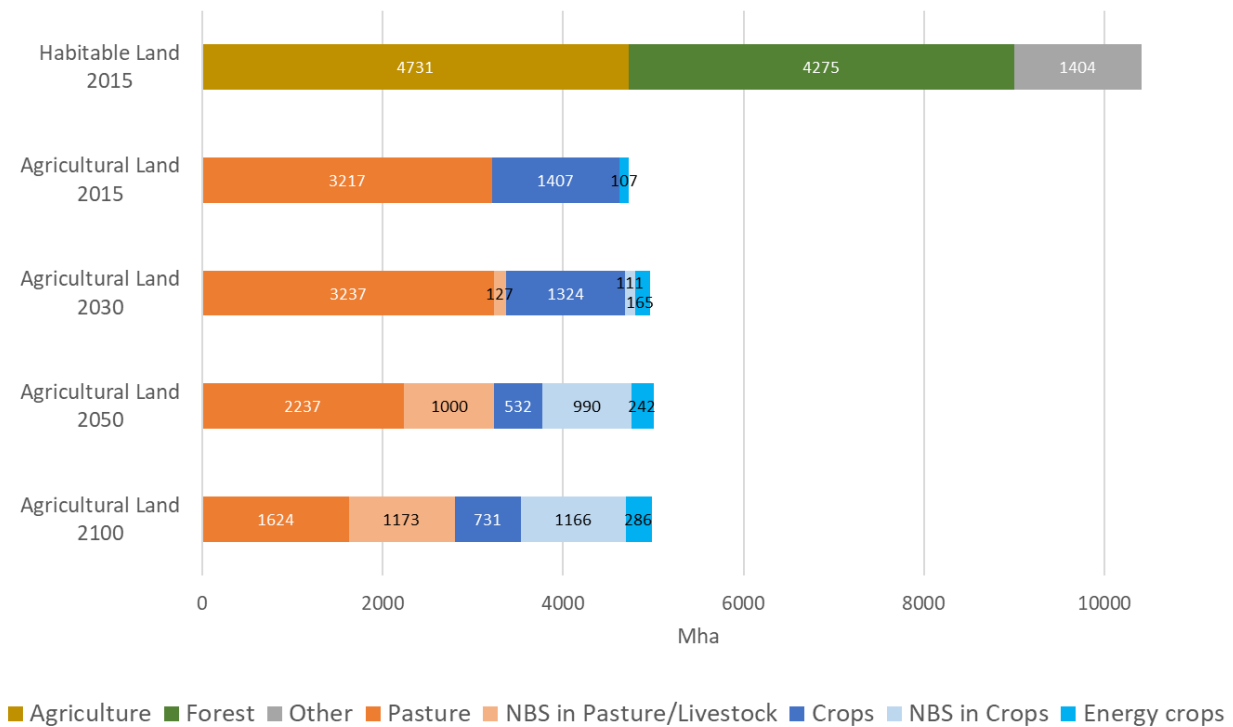
Figure 5. Projections for agricultural land use in the Sky scenario. Source: authors calculations.
