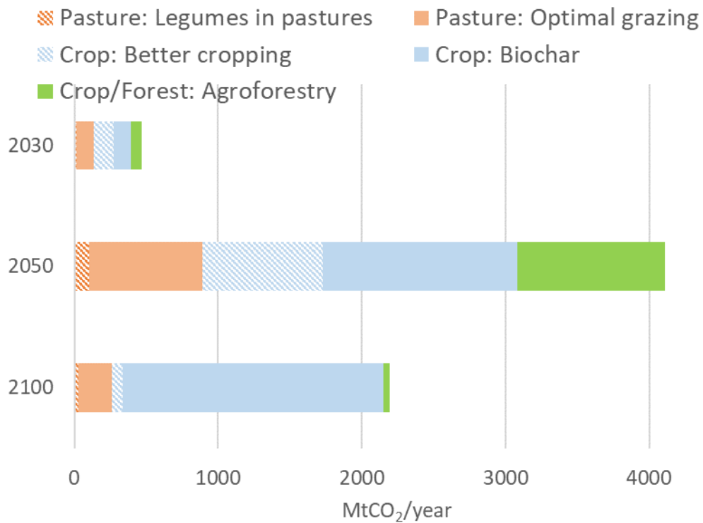
Figure 7. Projections for CO 2 sequestration in crops and livestock. Source: authors calculations.
