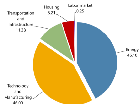
Figure 4. Canada-Announced Climate Measures, by Sector
