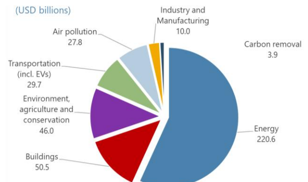
Figure 57. IRA Climate-Related Measures, by Sector
