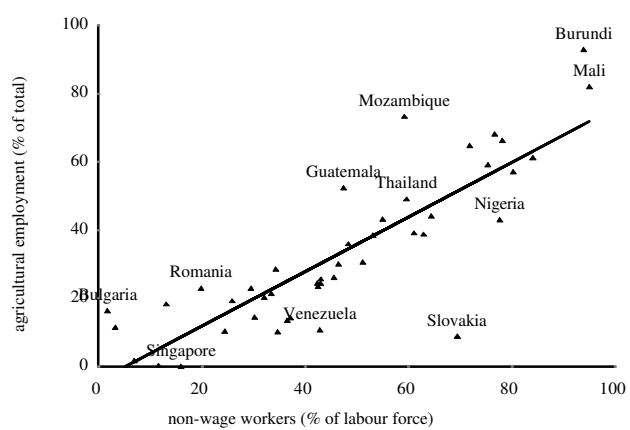
Figure 2.1 Non-wage workers and other development indicators
