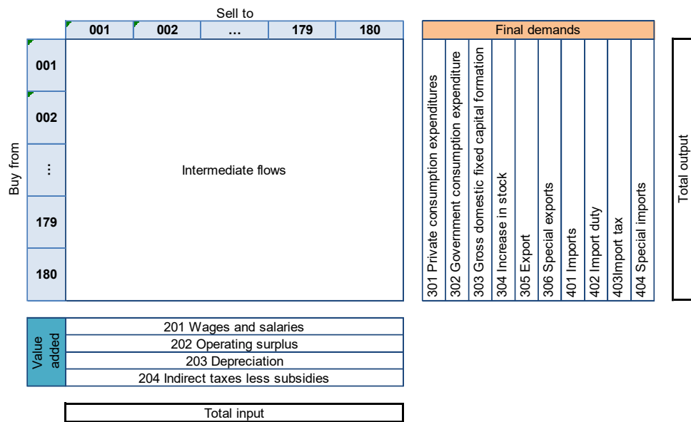
Figure 1. Overview of Thai I-O table (See Appendix 1 for detailed descriptions)
