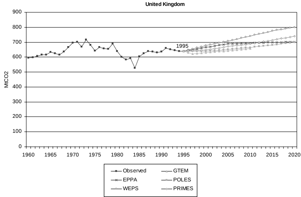
Fig. 9. CO 2 Emissions, 1960–2020 (in MtCO 2 ) (United Kingdom).
