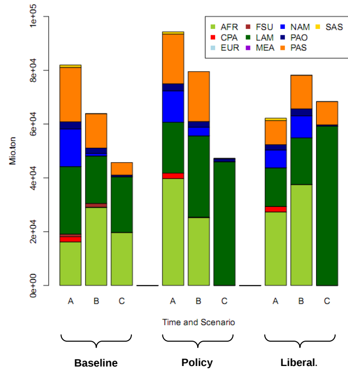
Figure 13: Carbon Emissions in time steps from 2005 to 2050 in three trade scenarios
