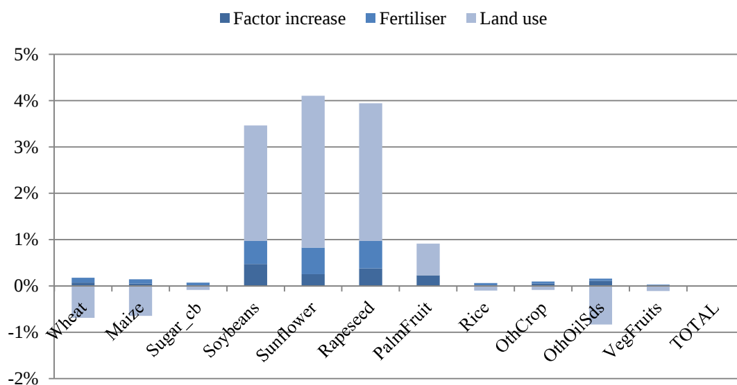
Figure 4. Increase in production at the world level in the “NAP” scenario, decomposed by source of growth: land expansion, fertilizers increaser and other factor increase.
