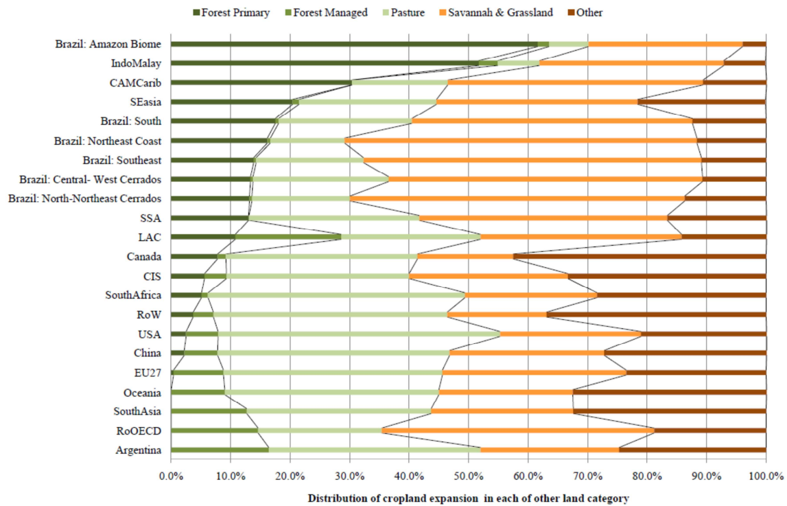
Figure 3. Distribution of cropland expansion across land use type categories for regions in the model.
