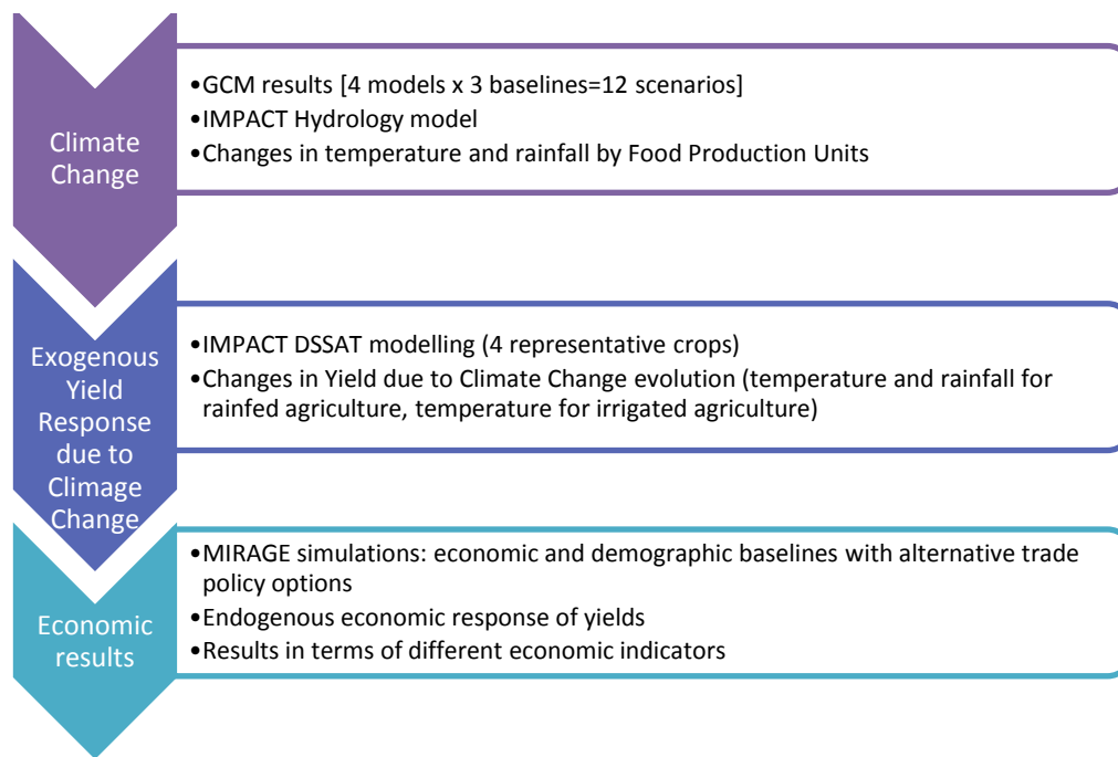
Figure 1 Modeling Framework
