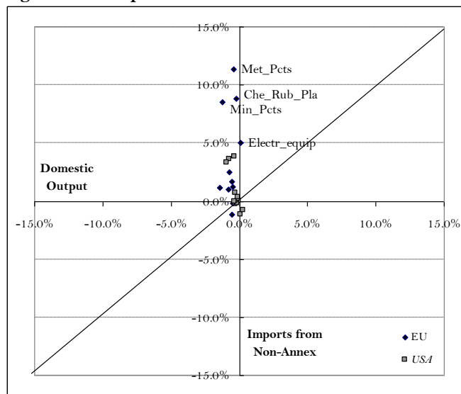
Figure 2 – Competitiveness effects for EU and the US in the KT scenario compared with baseline 2012
