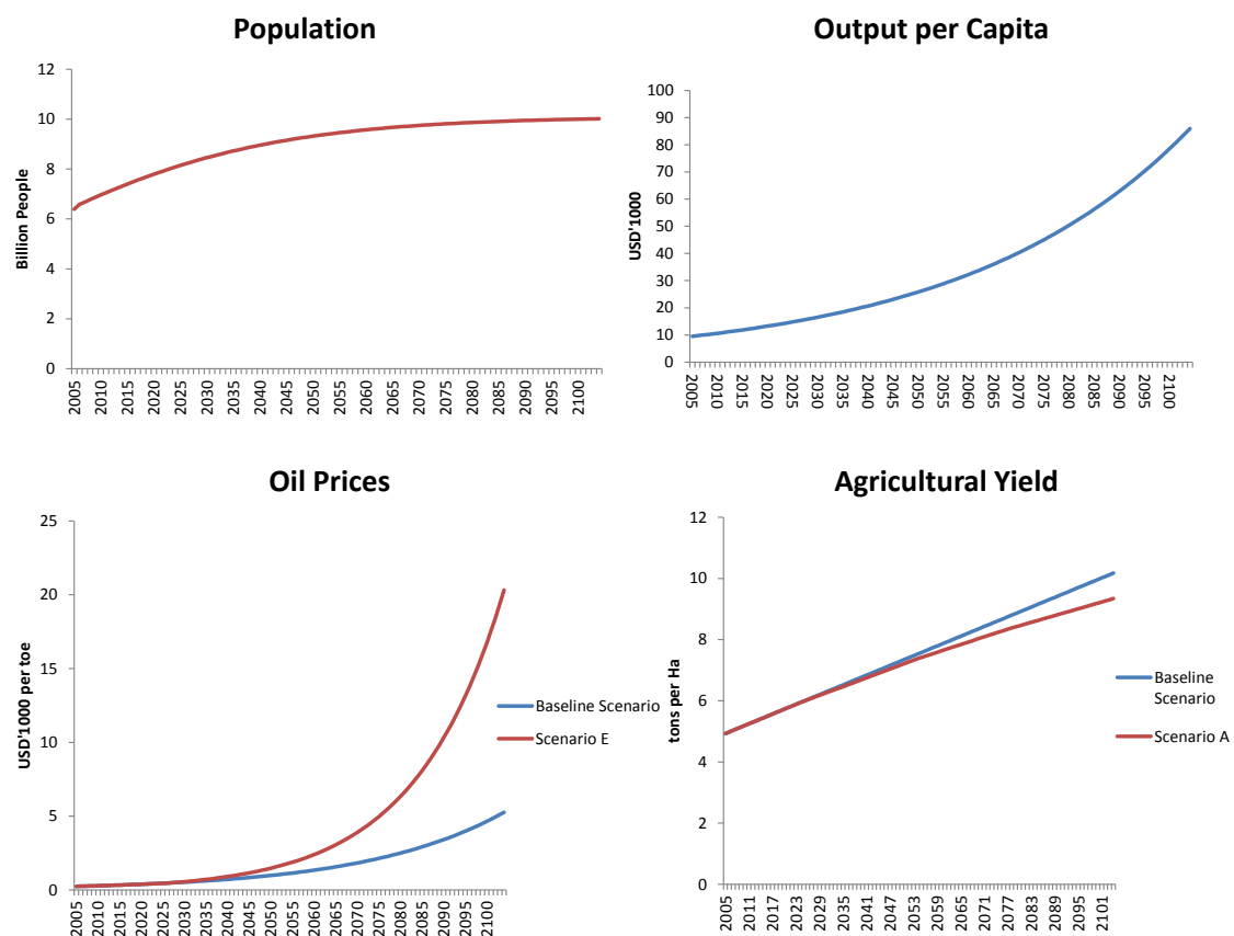
Figure C.1: Projections of Exogenous Variables, 2005-2104
