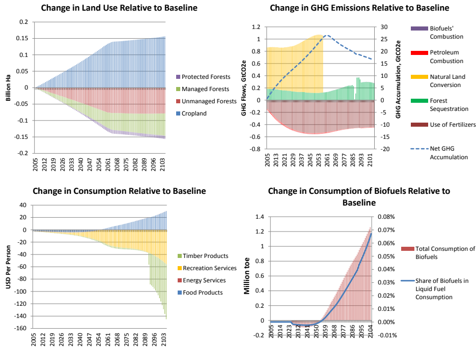
Figure D.2: Sensitivity Analysis: 50% Increase in Elasticity of Substitution between Agricultural Land and Fertilizers
