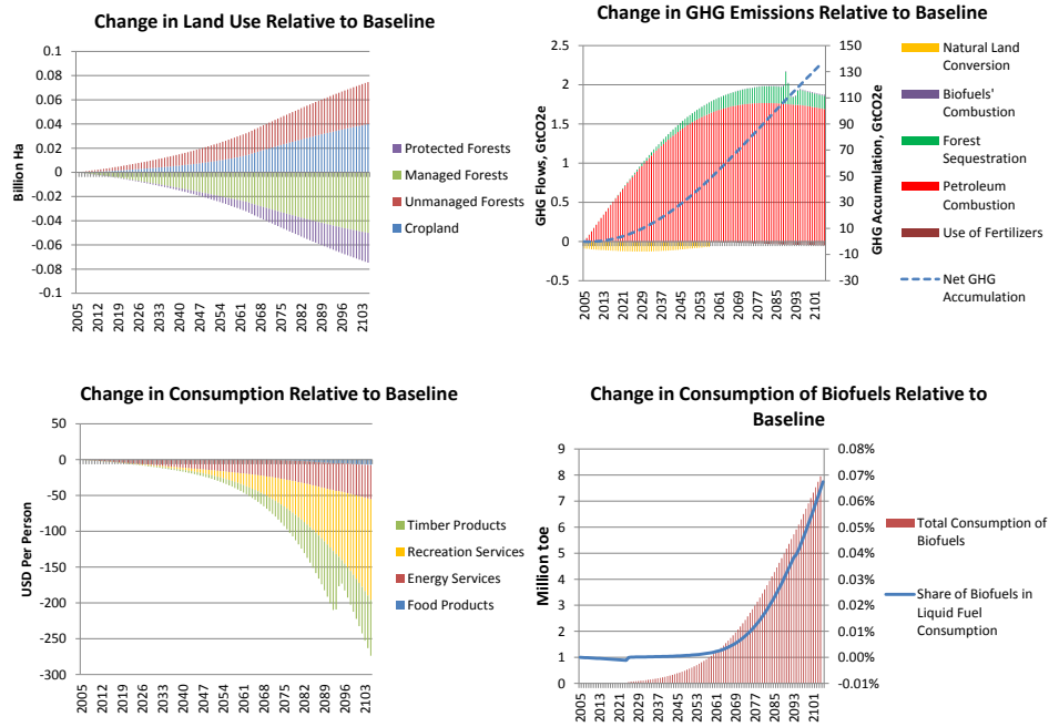
Figure D.5: Sensitivity Analysis: 50% Decline in Energy Efficiency Growth Rate per annum
