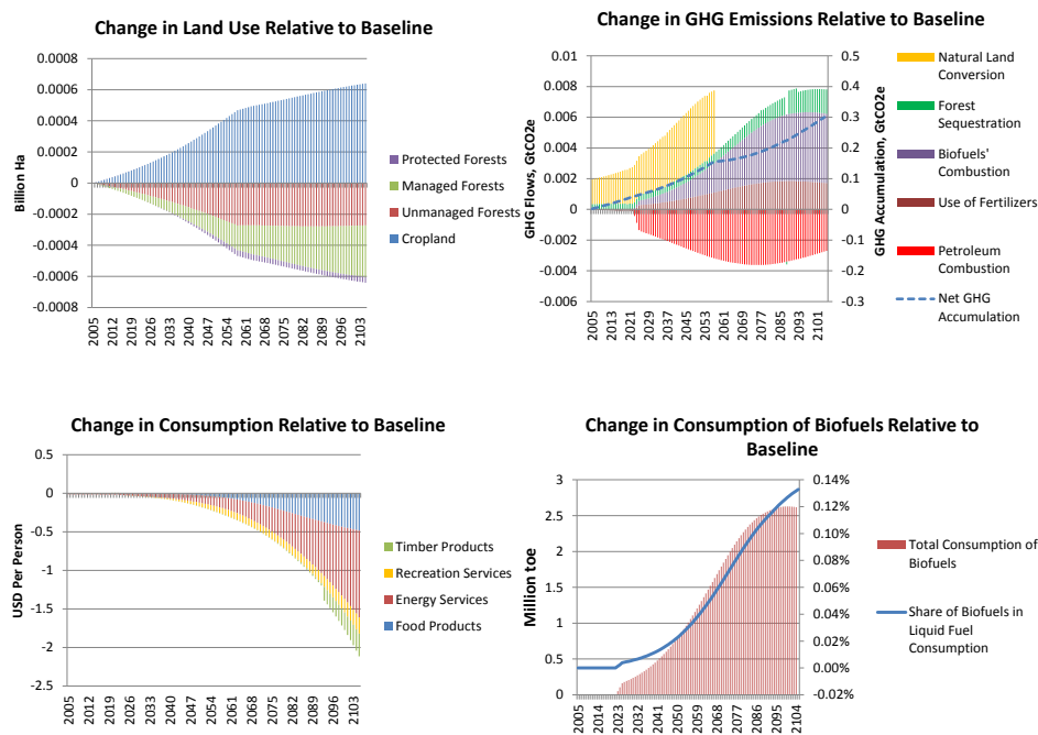
Figure D.4: Sensitivity Analysis: 50% Decline in Biofuels' Conversion Costs
