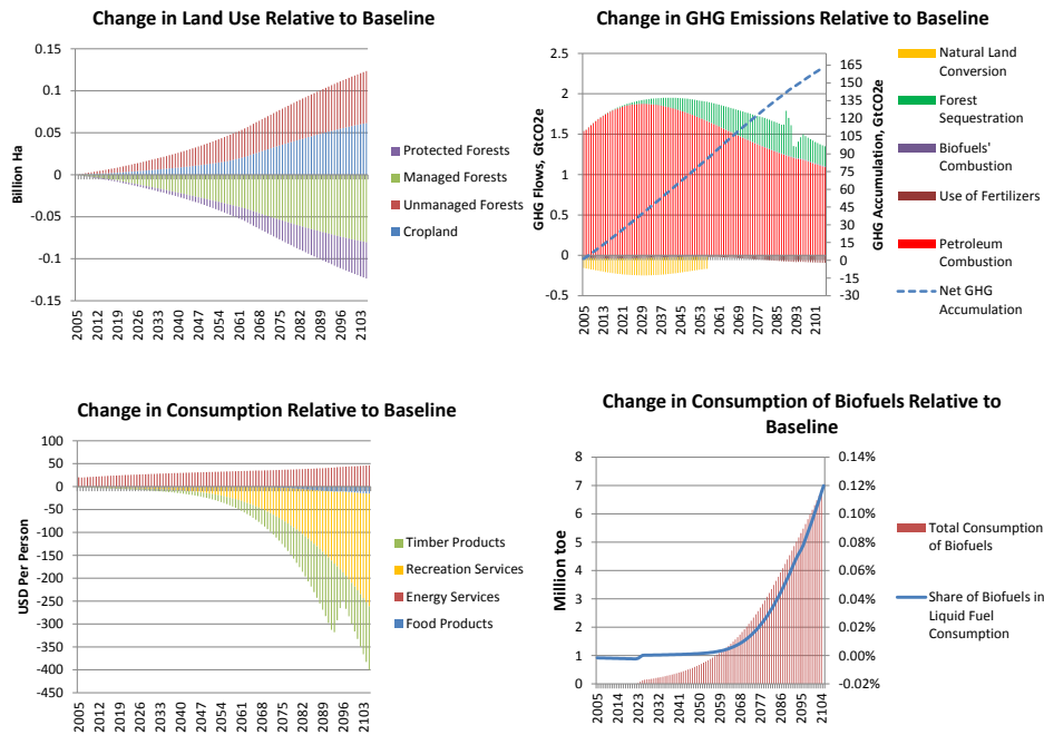
Figure D.6: Sensitivity Analysis: 50% Increase in AIDADS Marginal Budget Shares for Energy Services
