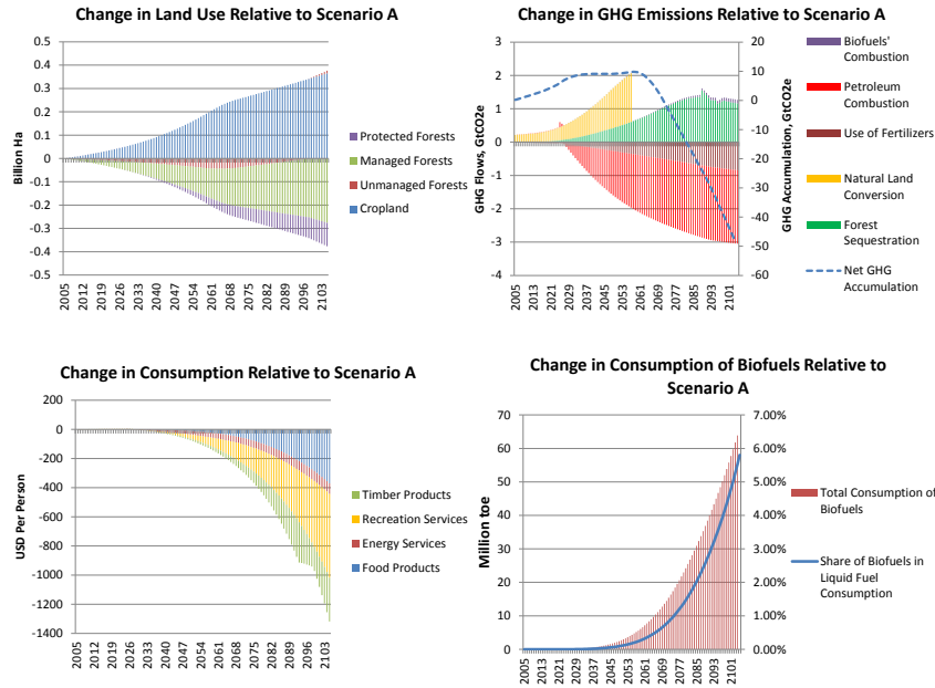
Figure 3: Scenario AE: Declining Agricultural Yield and Rising Fossil Fuel Costs
