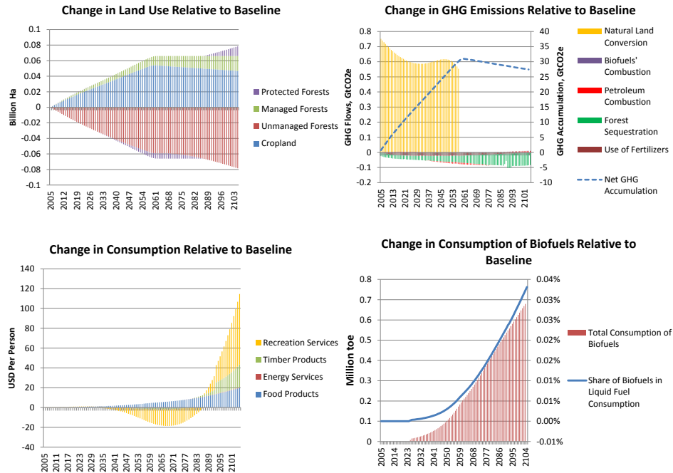
Figure D.1: Sensitivity Analysis: 50% Decline in Short Term Adjustment Costs of Natural Land Conversion
