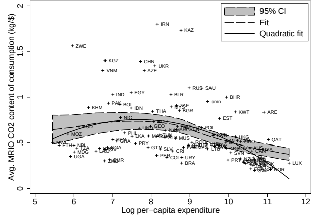
(c) Total \text{CO}_2 content of consumption
