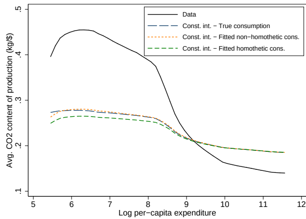
(b) Avg. MRIO CO 2 content of production
