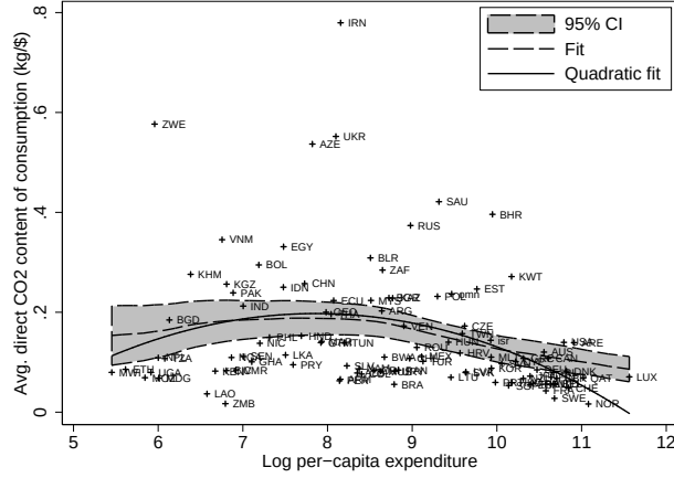
(a) Direct \text{CO}_2 content of consumption
