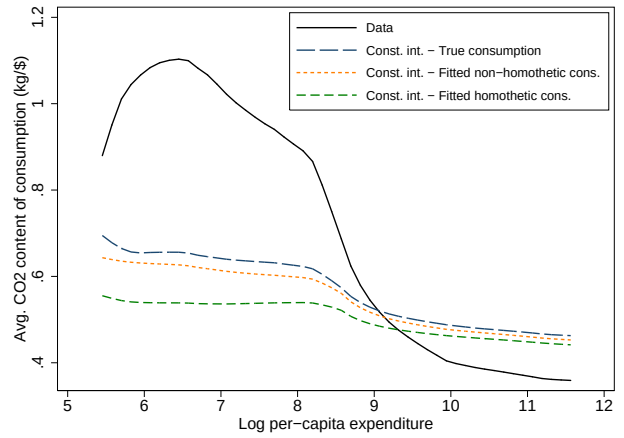
(c) Avg. MRIO CO 2 content of consumption
