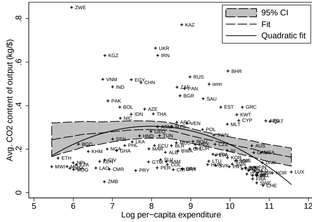
(b) Total \text{CO}_2 content of production
