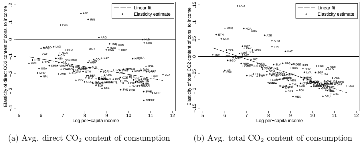
Figure 7: Elasticity of the CO_2 content of consumption to per-capita income
