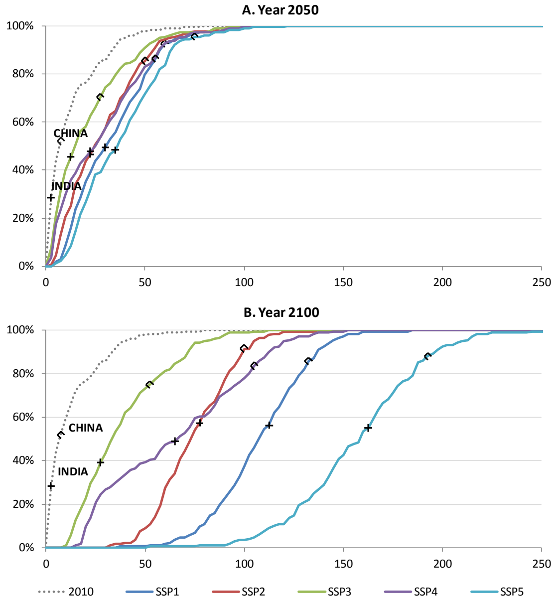
Figure 7. Distribution of income levels (Per capita GDP PPP (thousand USD 2005 per person))
