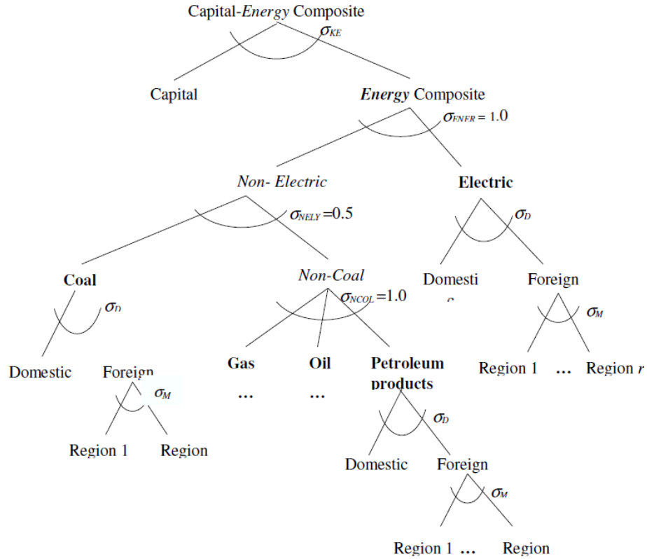
Figure 3 GTAP-E Capital-Energy Composite Structure
