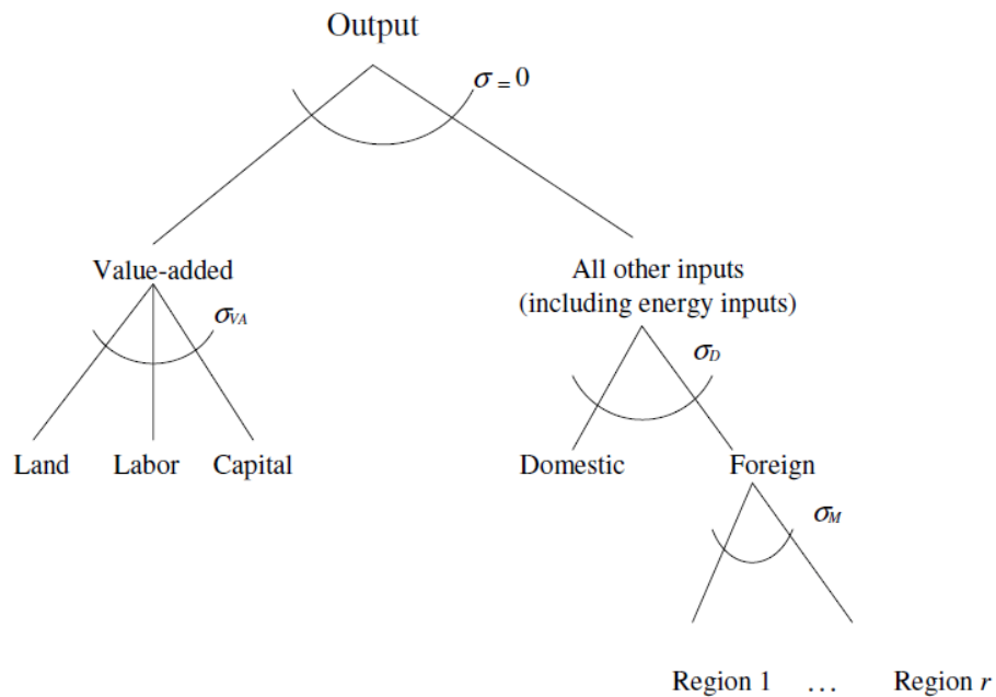
Figure 1 Standard GTAP Production Structure
