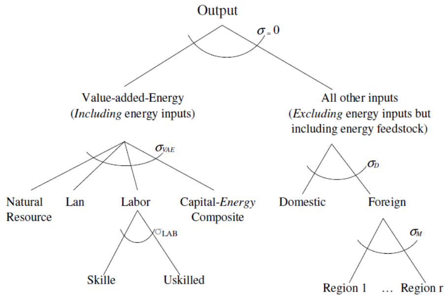
Figure 2 GTAP-E Production Structure
