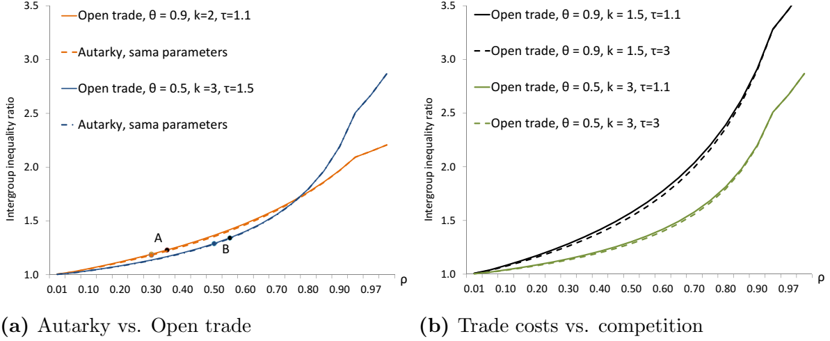
Figure 6: Intergroup inequality ratio with different parameters
