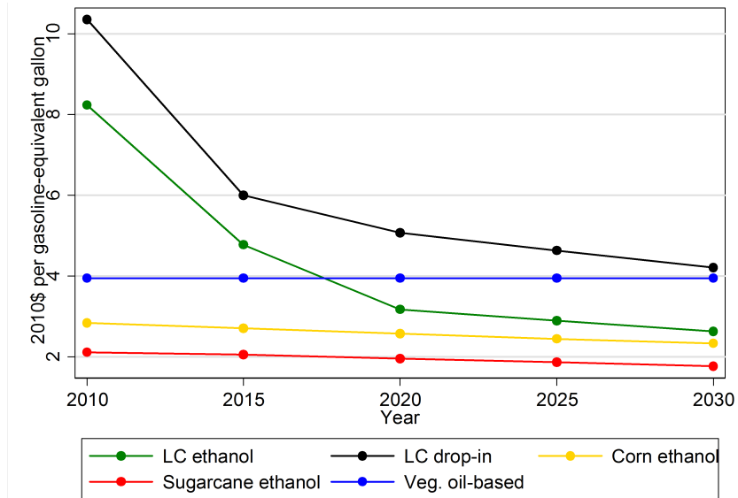
Figure 4. Benchmark biofuel costs in the US (for corn and LC ethanol and vegetable oil-based fuels) and Brazil (for sugarcane ethanol), 2010$ per gasoline-equivalent gallon.
