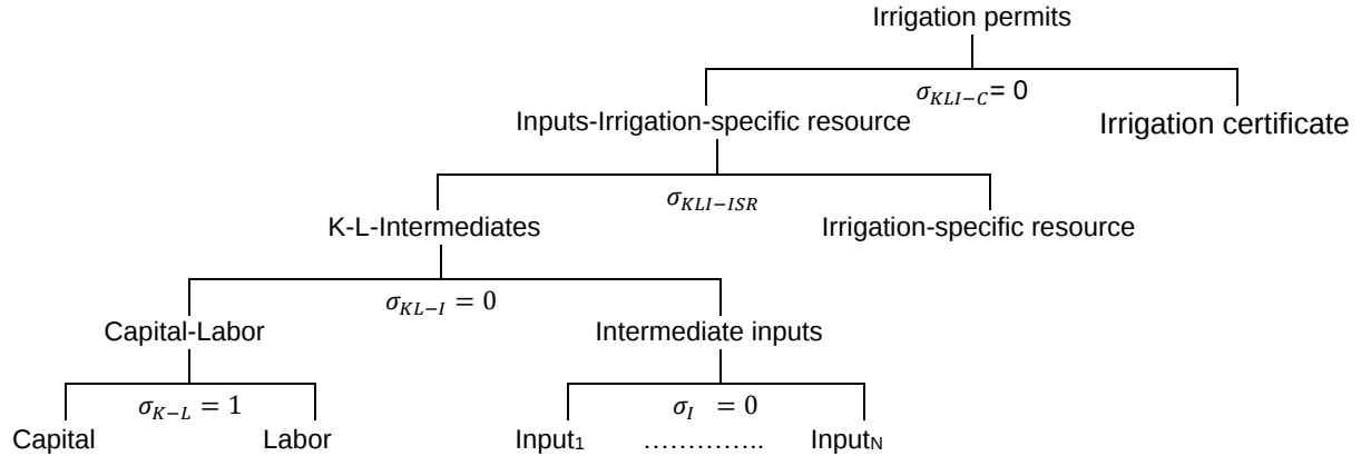
Figure 7. Production of irrigated land permits for each IRU in the EPPA model.
