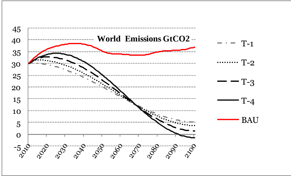
Figure 1: Global CO 2 emissions (energy only)
