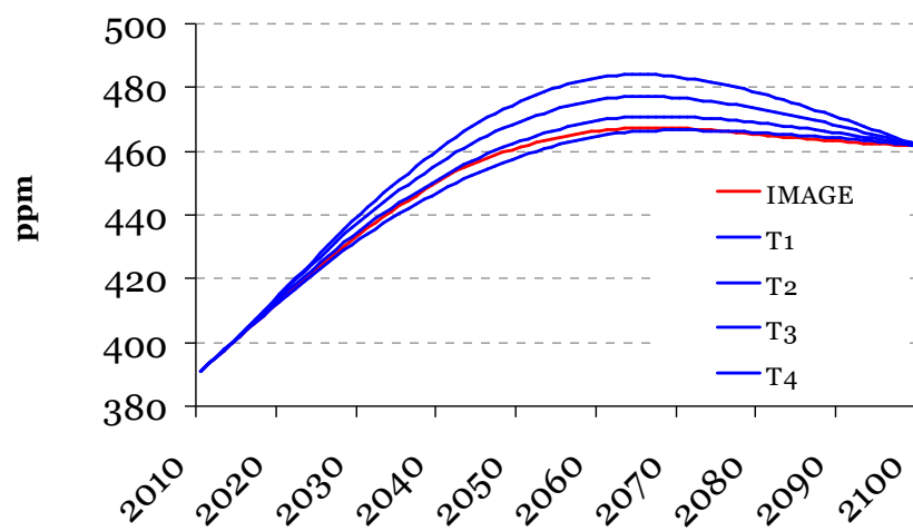
CO2 concentration
