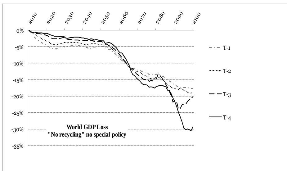
Figure 2: Global GDP variations between stabilization and reference scenarios (for the different emissions targets)
