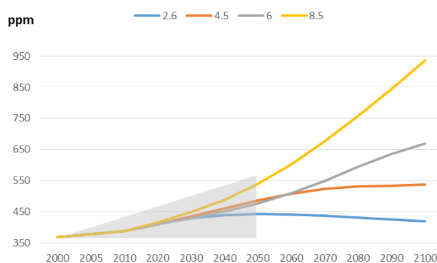
Figure 4 - CO 2 concentrations 2000-2100 by RCP. Concentrations are determined by the IMAGE, MiniCAM, AIM, MESSAGE models for RCP 2.6, 4.5, 6.0 and 8.5 respectively
