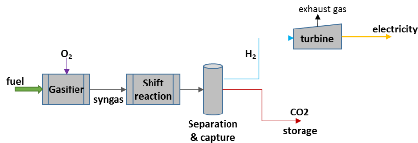
Figure 6. Pre-Combustion
