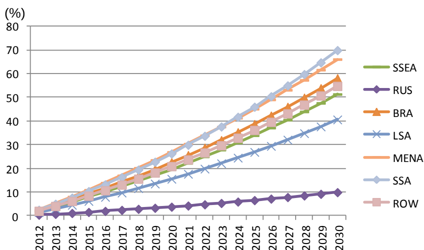
Figure 1 Changes in carbon emissions of countries without reduction targets under the Paris Agreement
