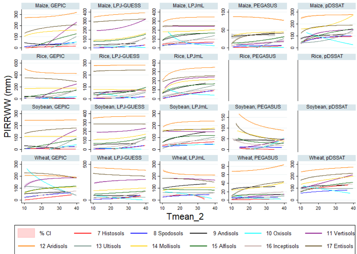
Figure 2. Effect of Tmean_2 on PIRRWW by crop and GGCM for the S1fpintsoil specification
