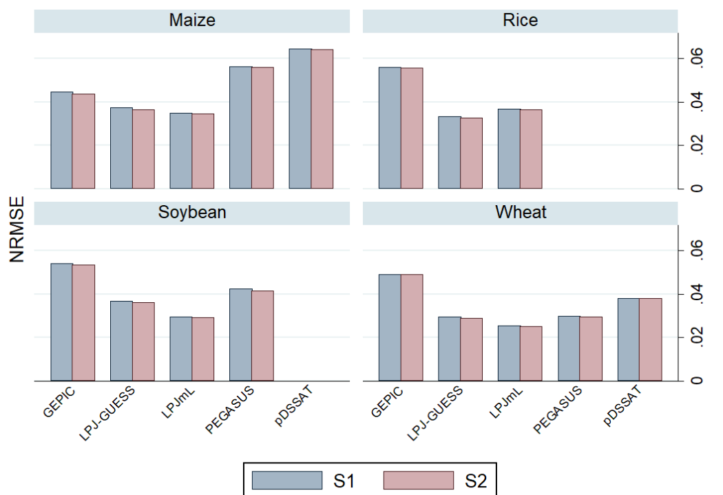
662 Figure A2. Goodness of fit of the irrigated yield statistical emulators by crop and GGCM (S1fpintsoil and S2fpintsoil 663 specifications)
