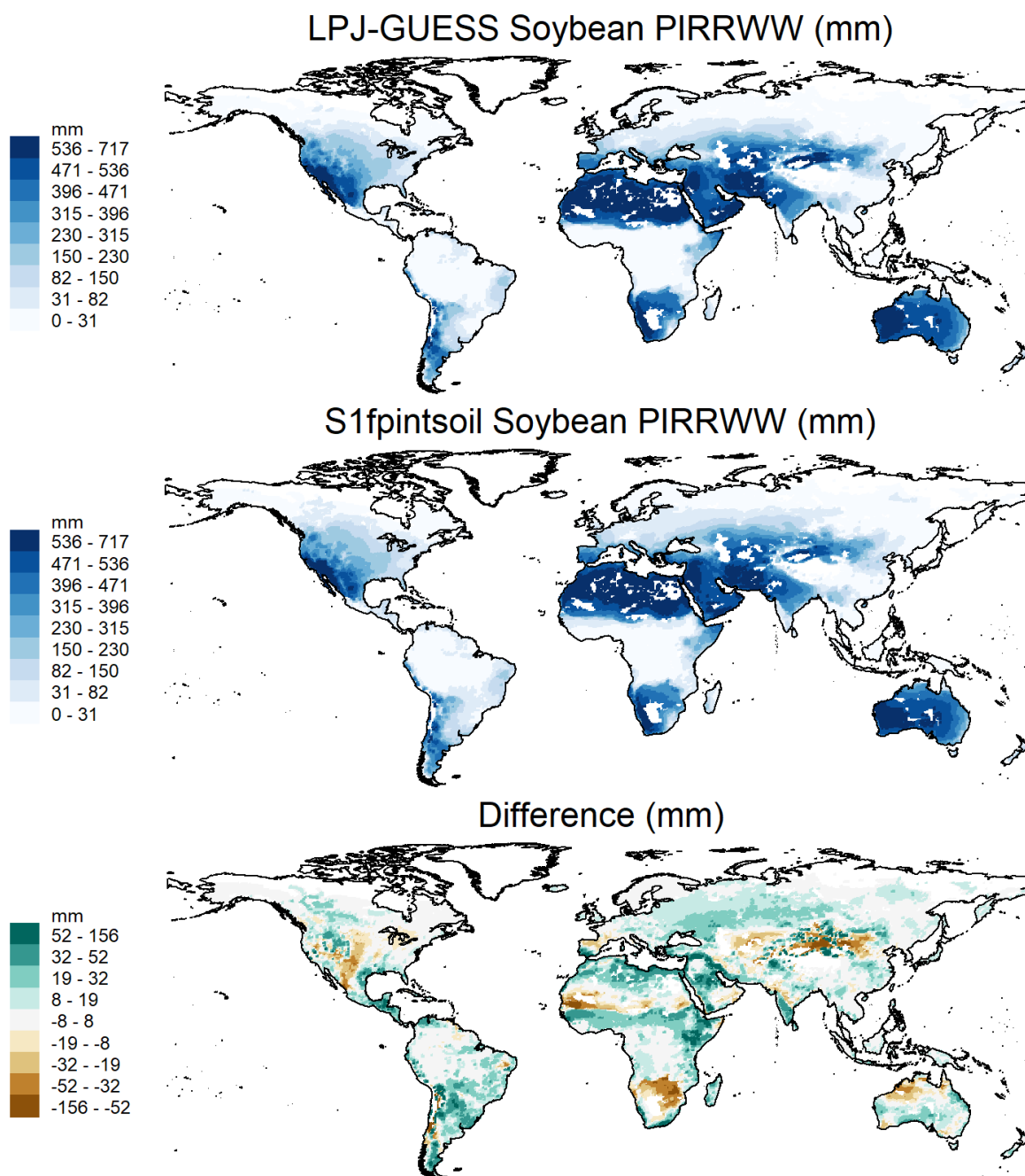
Figure H10. Irrigation water withdrawal for soybean averaged over 2090–2099 for the LPJ-GUESS model and S1fpintsoil specification
