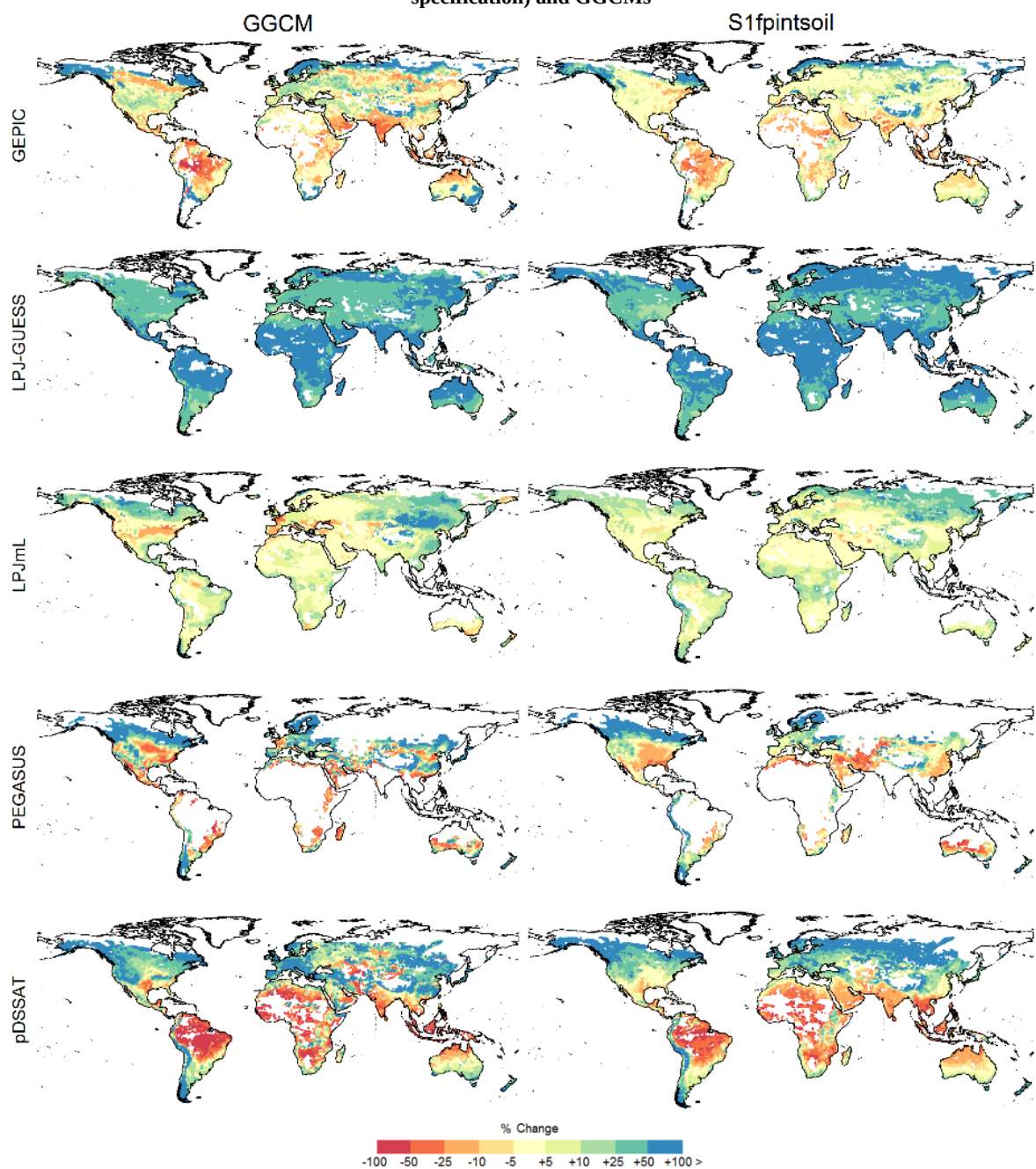
809 Figure G22. Changes in irrigated wheat yields from 2000s to 2090s estimated by the statistical emulators (S1fpintsoil 810 specification) and GGCMs
