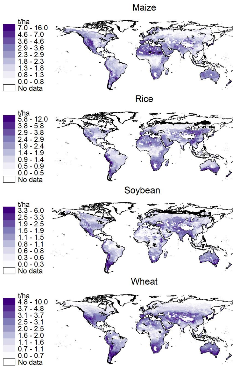
Figure G18. Irrigated crop yields ensemble error averaged over 2090–2099 across GGCMs at the global level
