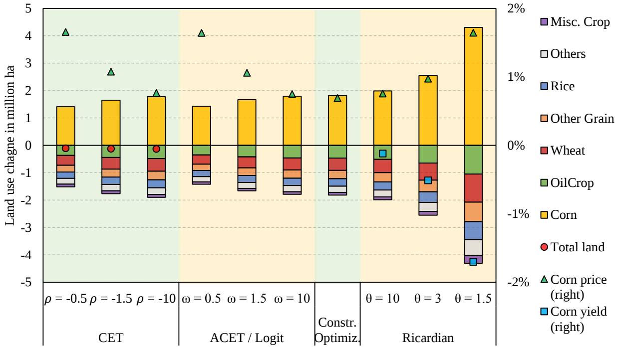
Figure 1 Comparison of land use change decomposition results, crop producer price change, and corn yield change across different land use modeling methods (GCAM crops not shown are aggregated into others)
