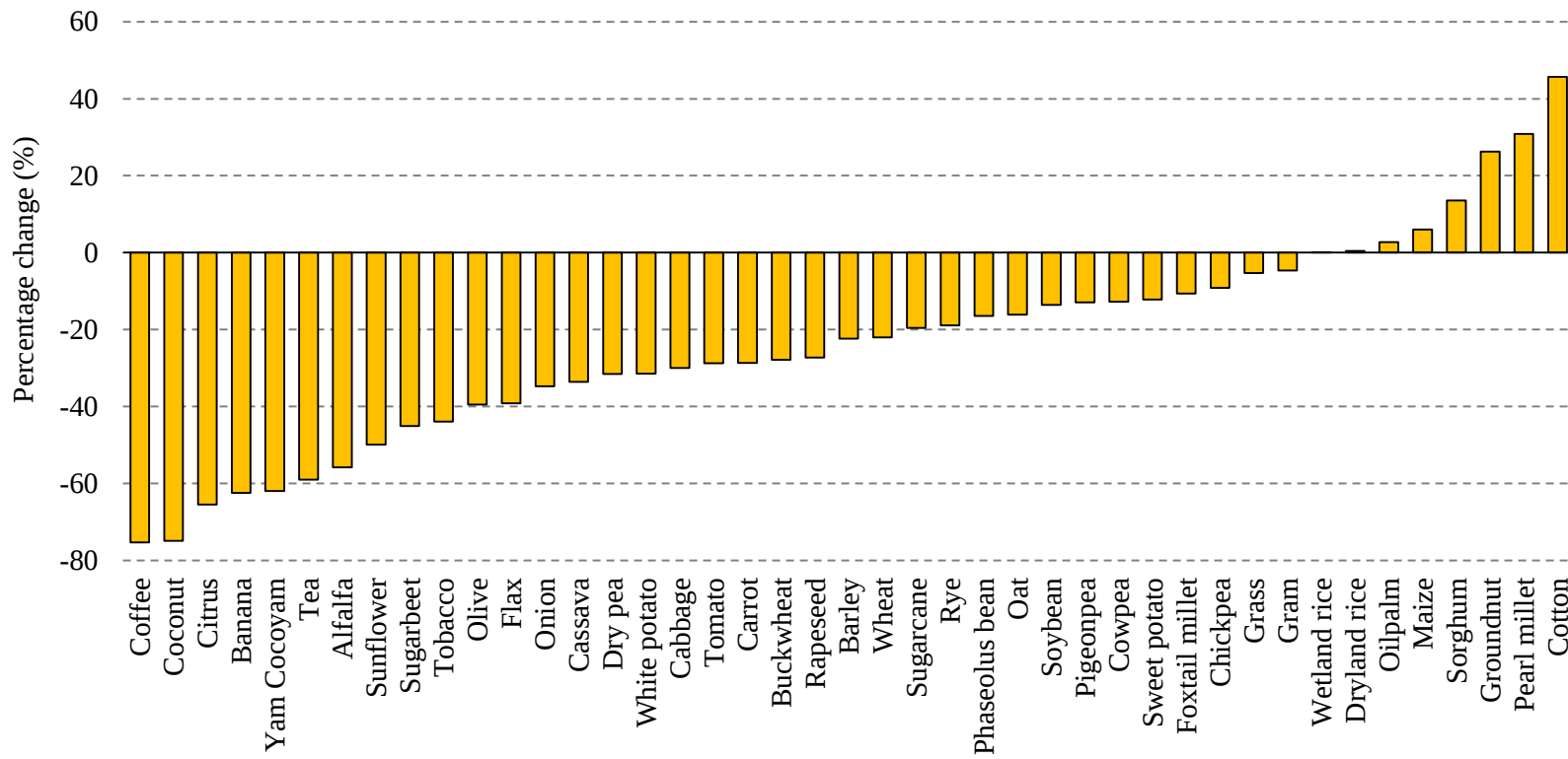
Figure A1 Climate change impacts on an average yield of GAEZ crops in the 2080s compared with the 1970s, estimated by GAEZ based on HadCM3-A1FI
