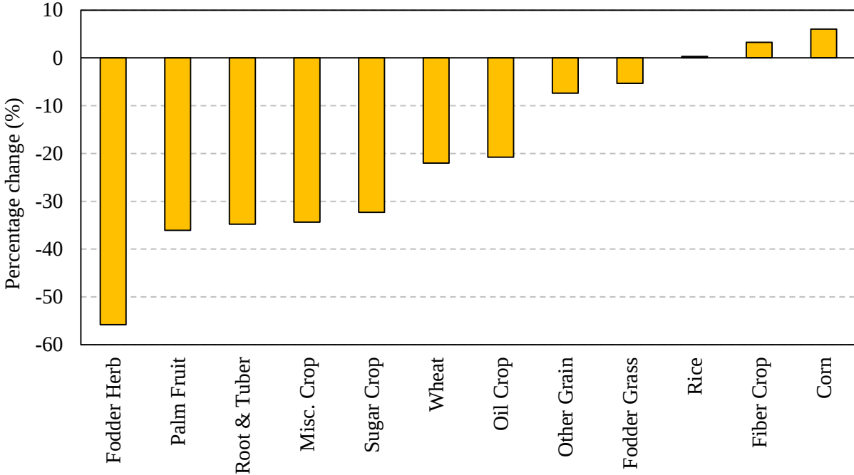
Figure 2 Climate change induced mean yield shift of GCAM crops in the HadCM3-A1FI scenario
