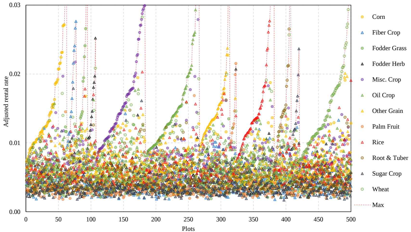
Figure A2 Calibrated maximum Frechet distribution of conversion cost adjusted rental rate ( \theta = 3 ), simulated with 500 plots. On each plot, the farmer picks the crop with the highest conversion cost adjusted rental revenue. The share of land use is calculated to the base data for the 12 GCAM crops.
