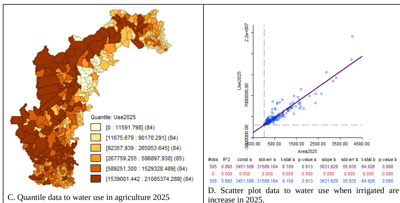
Figure 5. Policy deviation results for irrigated areas and water use in 2025
