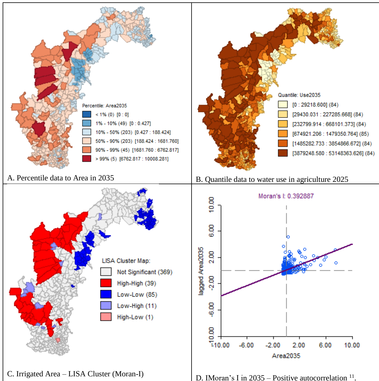
Figura 4. Policy deviation results for irrigated areas and water use in 2035.
