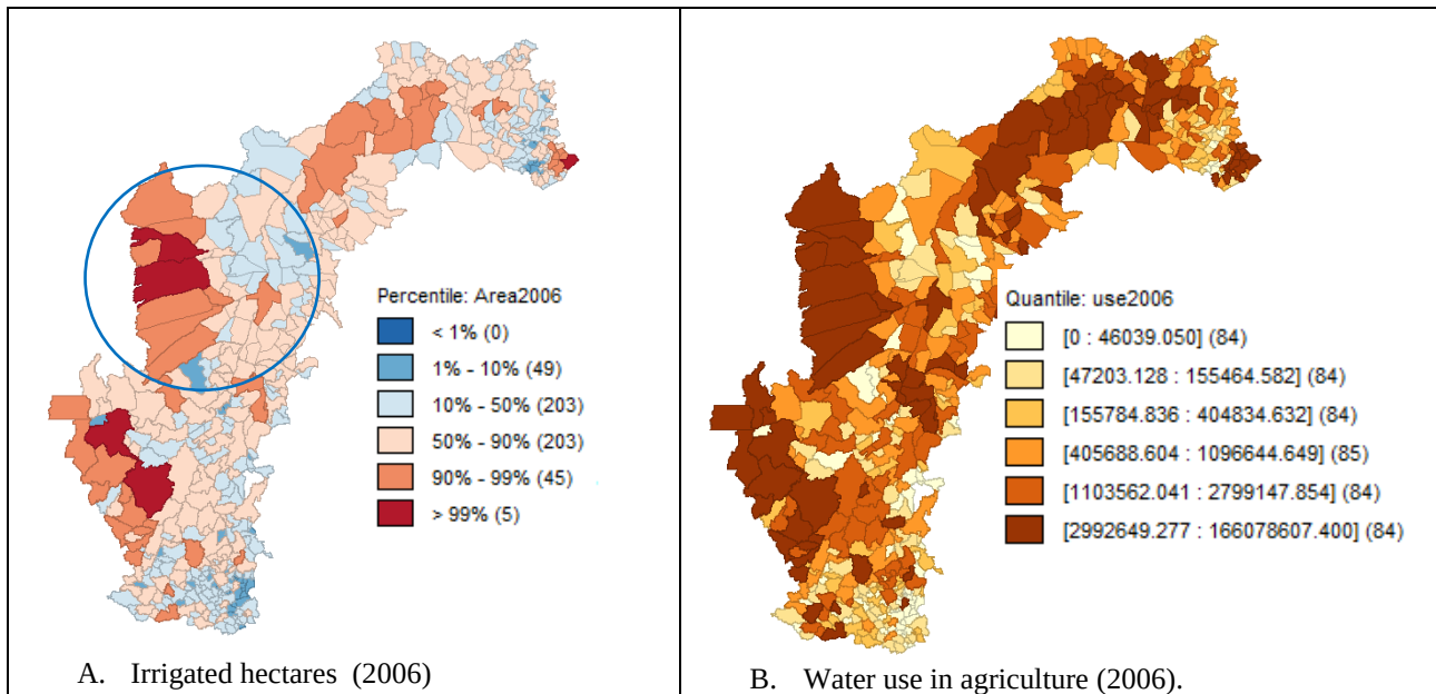
Figure 4. (A) Irrigated areas (hectares) by municipality in the São Francisco river basin in 2006. (B) Water use in agriculture.
