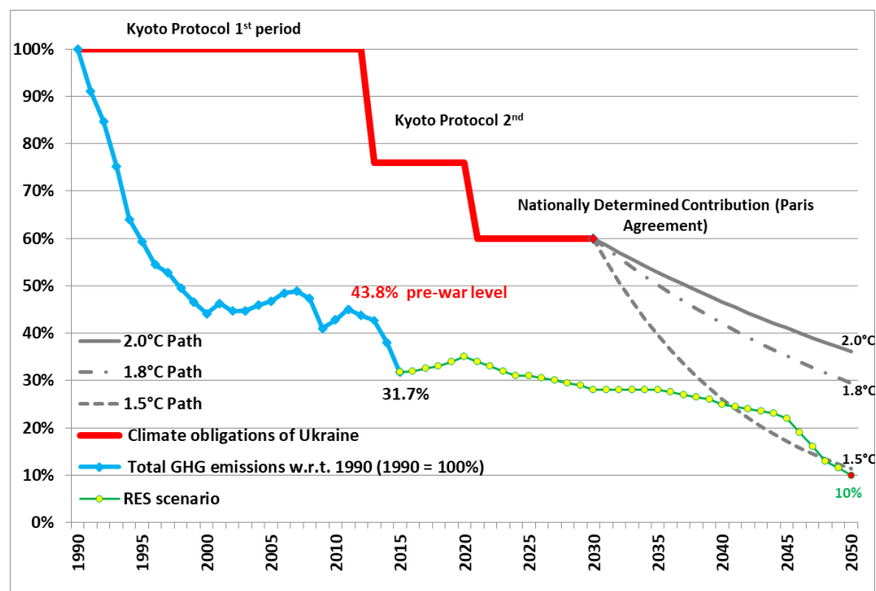
Figure 9. Emission under RES scenario and climate obligations of Ukraine
