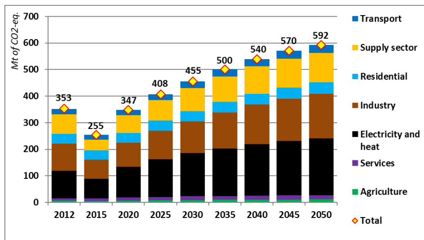
Fig. 7. Forecast of the GHG emissions in Ukraine according to the BaU scenario Source: Developed by authors using TIMES-Ukraine model.
