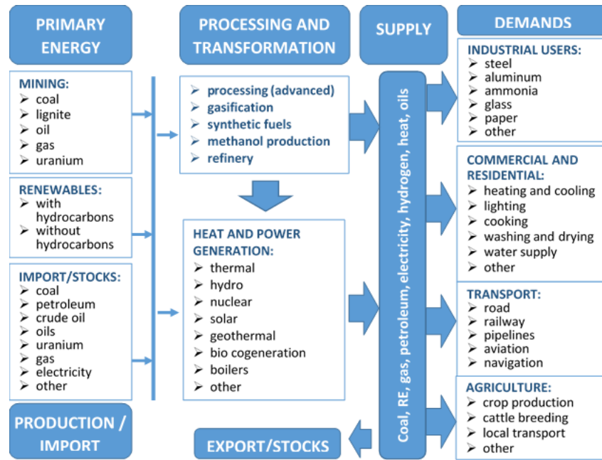
Figure 3. Representation of the energy system in TIMES-Ukraine model
