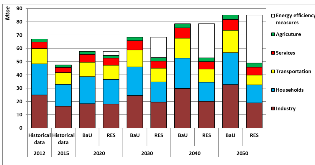
Figure 10. Final energy consumption by users under BaU and RES scenarios
