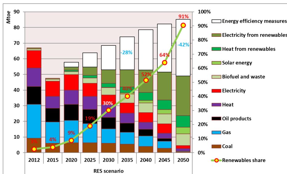
Figure 11. Final energy consumption by sources and renewables share under the RES scenario
