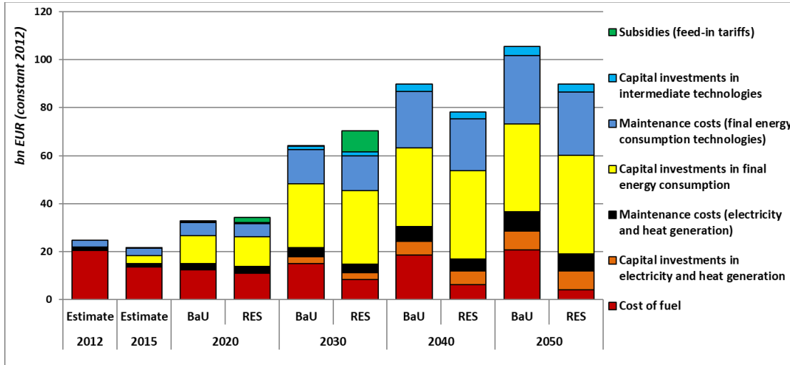
Fig. 14. Annual energy system costs under BaU and RES scenarios
