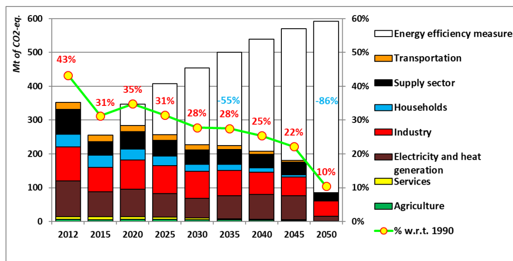
Fig. 13. GHG emission under the RES scenario
