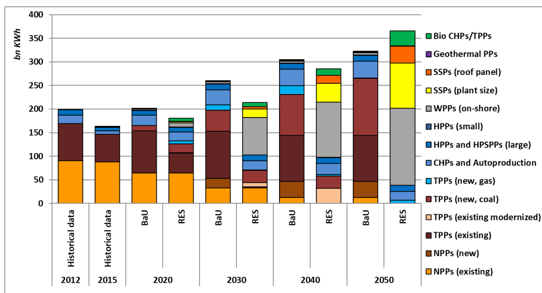
Fig. 12. Electricity generation mix under BaU and RES scenarios
