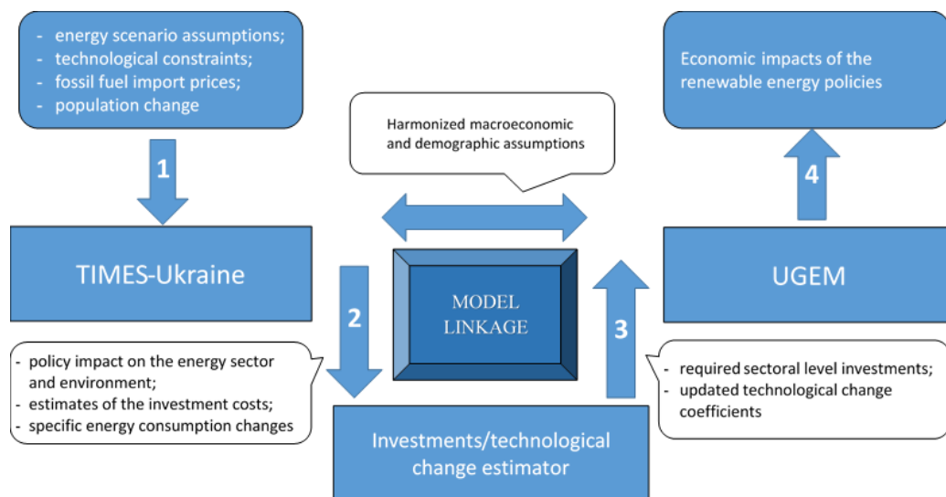
Figure. 6. TIMES-Ukraine and UGEM models linkage
